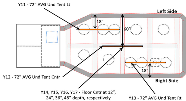
Fig. 6 Sensor locations of 72-in.-long averaging RTDs between tent bottom and mine floor strata, and 48-in.-long RTDs measuring mine floor strata temperature at various depths
