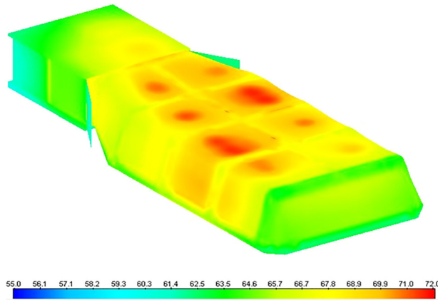
Fig. 13 Final RA surface temperature contour plot (simulated)
