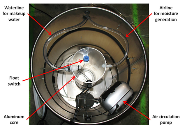
Fig. 3 Inside view of a simulated miner
