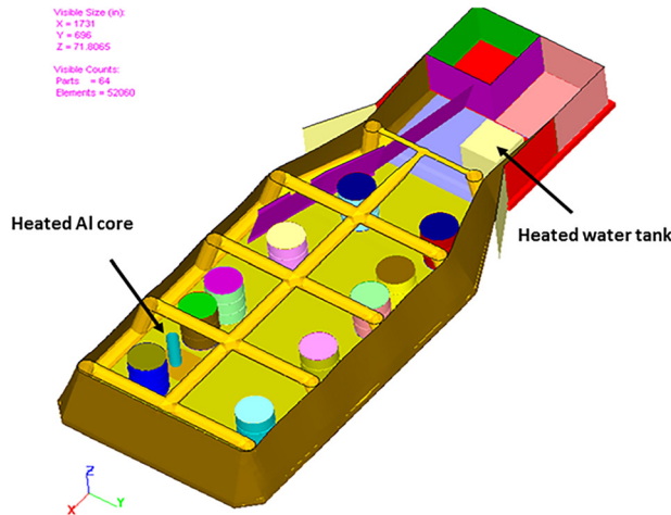
Fig. 10 Cut-away view of mine shelter with ten barrels (simulated miners) and two auxiliary heaters
