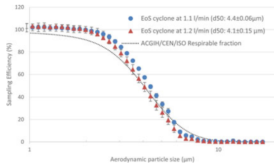
Figure 3. Sampling efficiency of EoS cyclone at the flow rates of 1.1 and 1.2 l min -1 together with ACGIH/CEN/ISO respirable convention.
