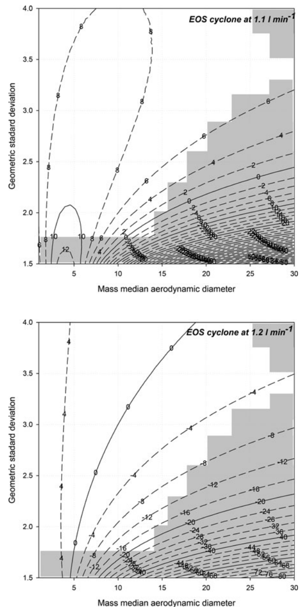
Figure 4. Bias maps of measured EoS cyclone performance at flow rates of 1.1 and 1.2 l min -1 compared to ACGIH/CEN/ISO respirable convention. Shaded area represents extreme particle size distributions, which are not included when assessing performance.
