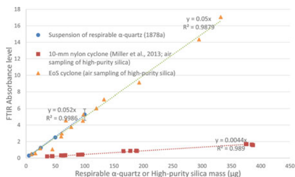
Figure 6. Comparison of calibration curves for the quartz quantification model for samples prepared in three different methods.
