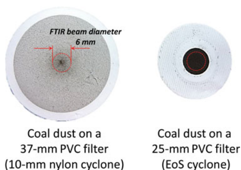
Figure 5. Comparison coal dust deposition area between 10-mm nylon cyclone (37-mm PVC filter) and EoS cyclone (25-mm PVC filter). Dotted line of circles indicate 6-mm beam diameter of portable FTIR.
