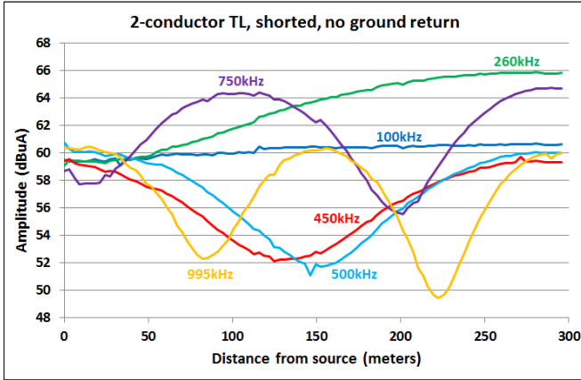
Fig. 8. Line current distribution – 2-wire TL, no ground connected
