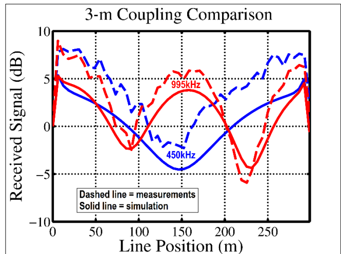
Fig. 12. Comparison of line to antenna coupling measurement vs. simulation
