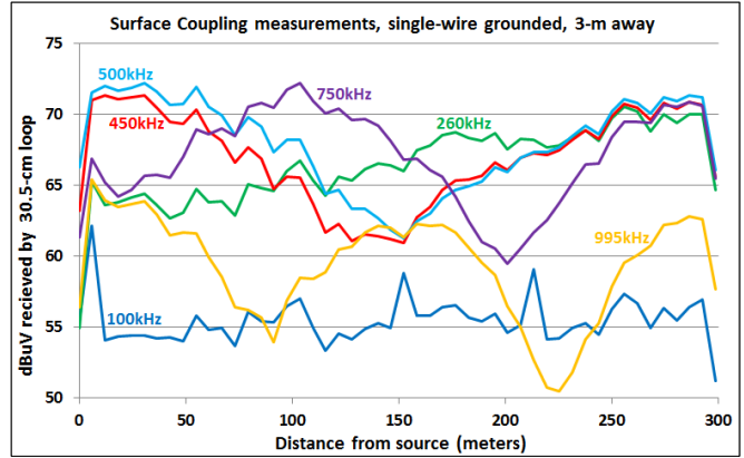
Fig. 11. Surface antenna coupling – 1-wire TL, connected to ground
