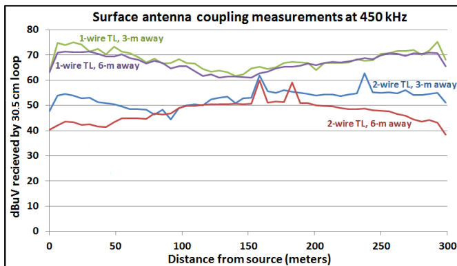
Fig. 10. Surface antenna coupling – 450 kHz, single-wire vs. 2-wire TL, loop antenna at 3-m vs. 6-m away from the TL, both shorted
