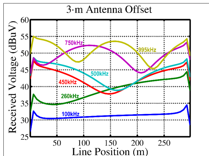
Fig. 4. Coupling simulation of a single conductor connected to ground
