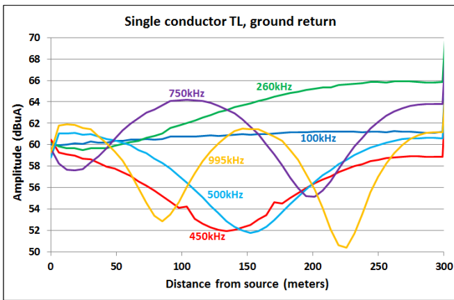
Fig. 9. Line current distribution – 1-wire TL, connected to ground
