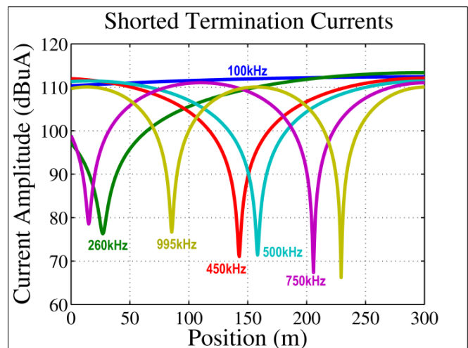
Fig. 3. Simulation result of line current distribution for a single conductor connected to ground
