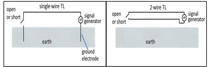
Fig. 6. TL test configurations
