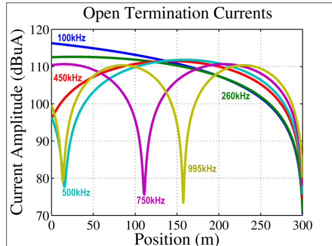
Fig. 2. A simulation result of line current distribution for an open TL
