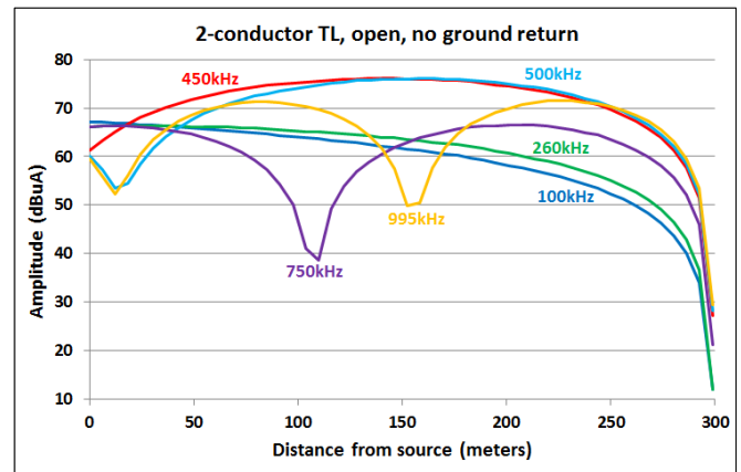
Fig. 7. Line current distribution – 2-wire TL, no ground connected
