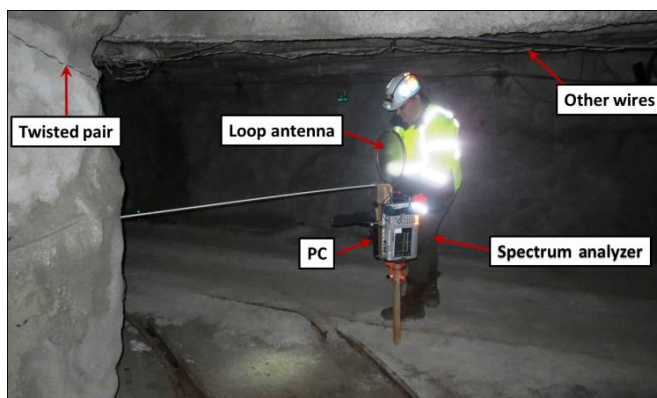
Fig. 13. Underground transmission line coupling measurements
