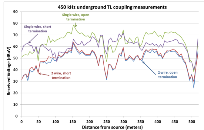
Fig. 14. Underground coupling measurements at 450 kHz
