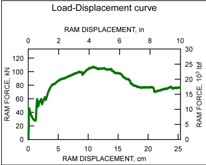
Figure 15. HEHD panel test load versus displacement curve.
