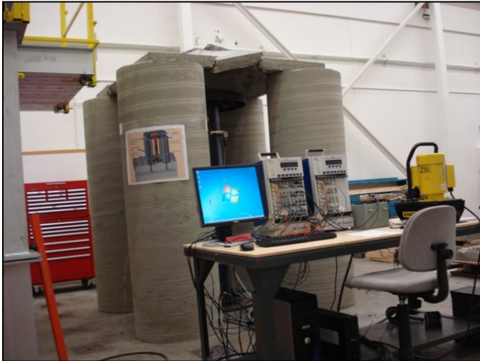
Figure 6. High-Energy, High-Displacement (HEHD test machine) in operation.
