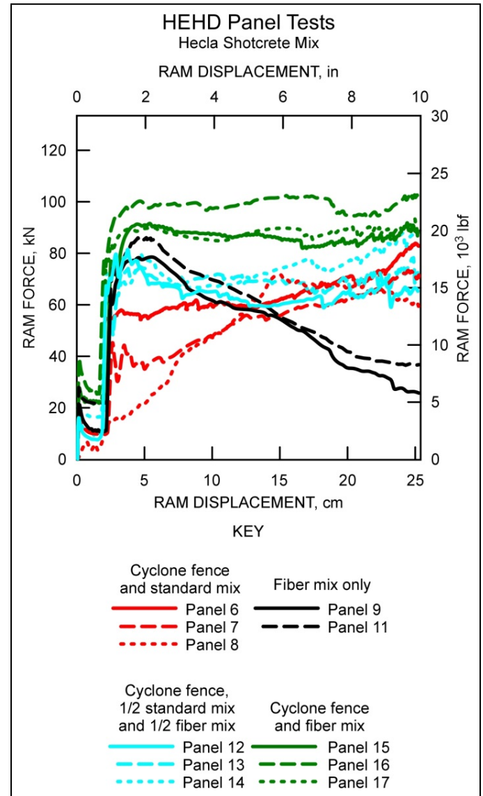
Figure 21. Load-displacement curve for mine specified sprayed panels.
