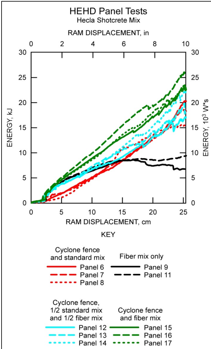
Figure 22. Energy-displacement curve for mine specified sprayed panels.
