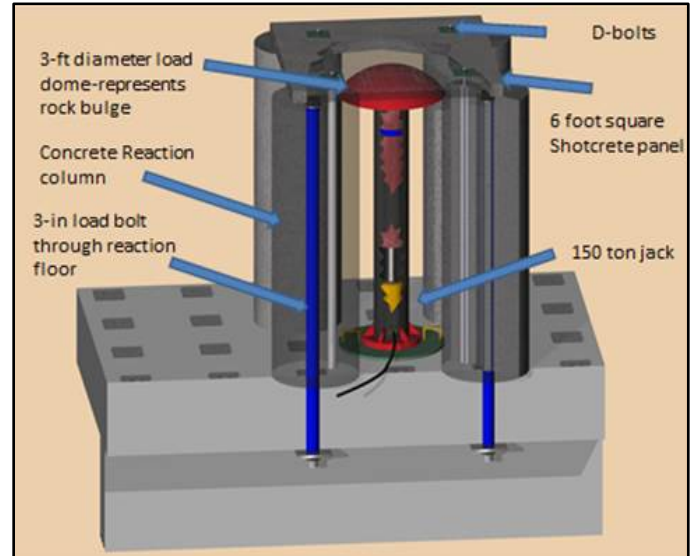
Figure 4. High-Energy, High-Displacement (HEHD) test machine design.
