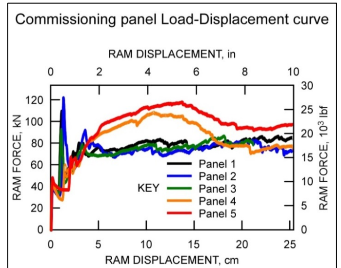
Figure 19. Load-displacement curves from HEHD panel tests.
