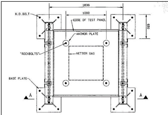
Figure 2. Plan view of panel testing frame, after Kirsten [1993].
