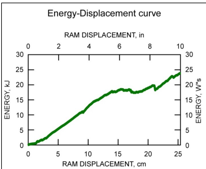
Figure 17. Energy versus displacement curve from HEHD test.
