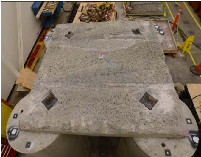
Figure 7. HEHD panel with in-mine roof bolt pattern.
