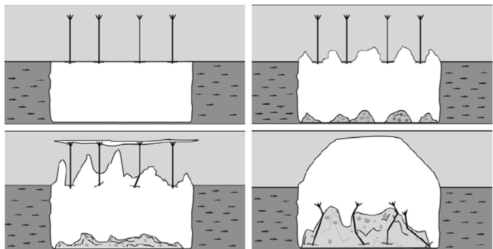
Fig. 10 Moisture-sensitive rock unraveling between the roof bolts and leading to a massive roof fall (from Molinda and Mark 2010)
