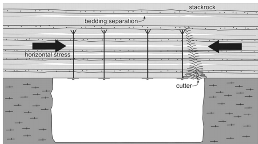
Fig. 4 Cutter formation as a result of high horizontal stress (from Molinda and Mark 2010)
