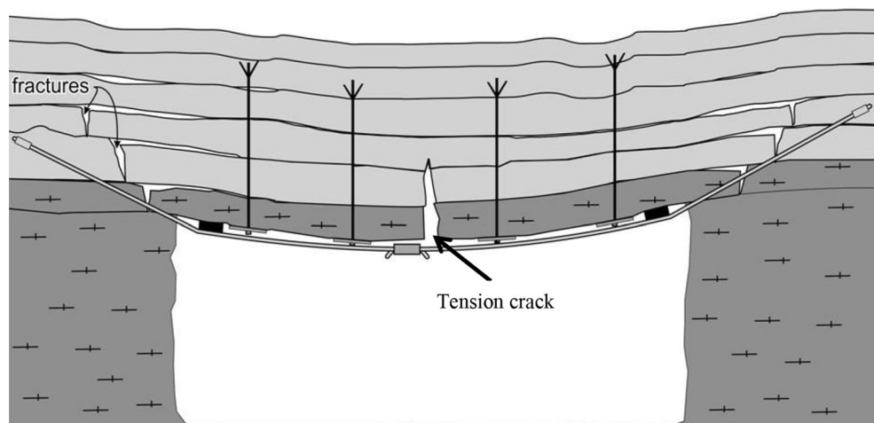
Fig. 8 Cross section of entry showing two modes of failure caused by sagging roof (from Molinda and Mark 2010)
