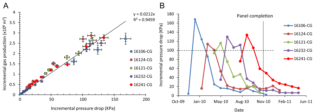
Fig. 11. Incremental gas production and formation pressure drop relation (A) and the history of change in pressure drop (B) during mining of the E-1 panel. The error bars in 10-A show 10% error margin of the value of the data points, whereas the 100 KPa level in B show the limit up to which the relation is linear for all GGVs.
