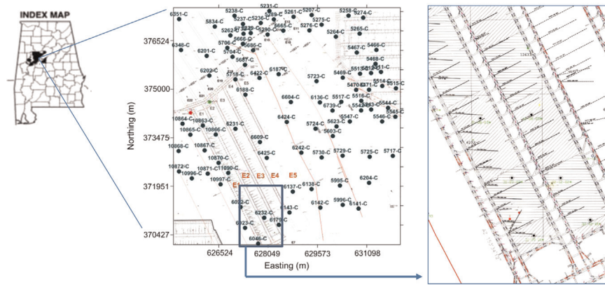
Fig. 2. Location of study area and a plan view with vertical degasification wellbore locations, mine outline, and major geologic structures with vertical displacements. The figure on the right is an expanded section of the panels that shows the horizontal, in-seam degasification boreholes.
