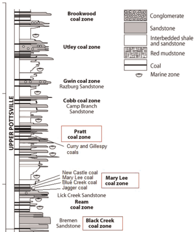
Fig. 3. Stratigraphic section of the Upper Pottsville Formation in the Black Warrior basin.
