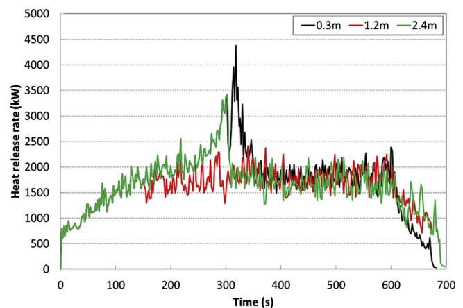
Fig. 7 – Heat release rates for different sprinkler locations.
