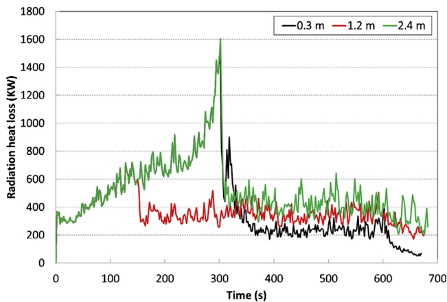
Fig. 12 – Radiation heat loss for different sprinkler locations.
