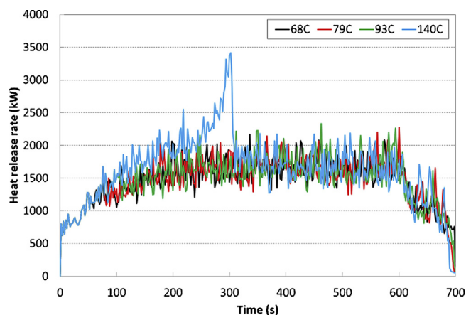
Fig. 17 – Heat release rates for different activation temperatures.
