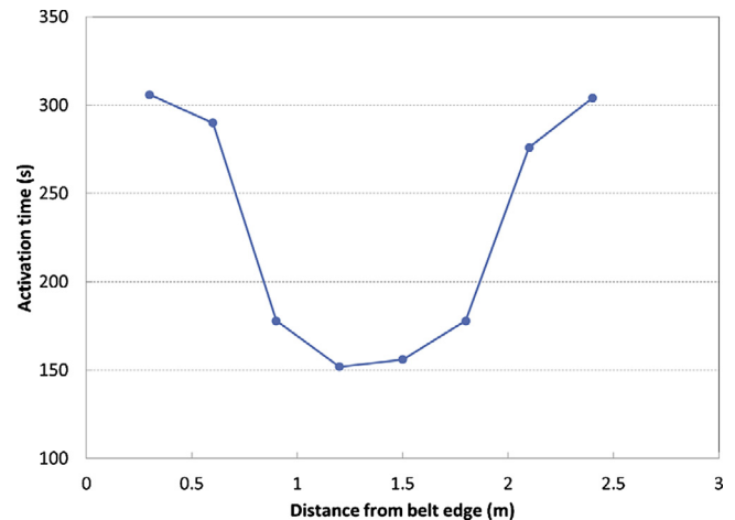
Fig. 6 – Activation times for the first sprinkler at different locations.
