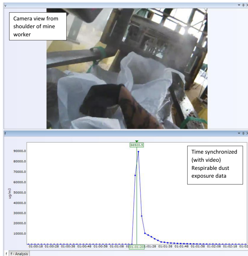
Fig. 6 Use of EVADE software (bulk bagger) linking the activity (worker approaching bulk bag after filling to begin tying the bag) to the dust exposure peak
