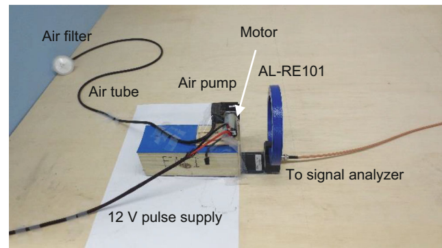
Fig. 4 Motor with its one side (side 3) sitting on test platform
