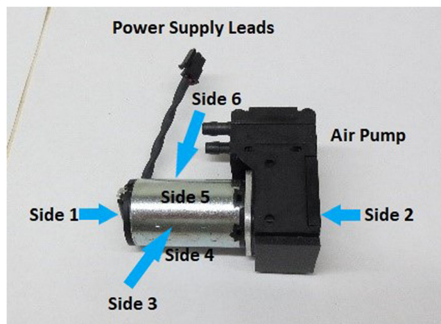
Fig. 3 Assembly of air pump and motor (side 4 on the bottom of the motor)
