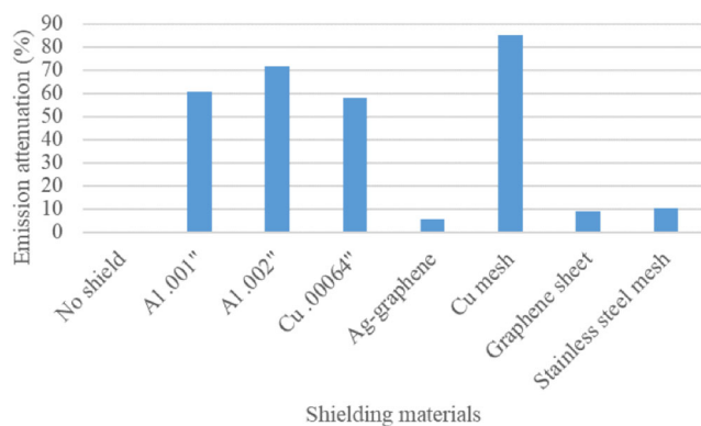
Fig. 9 Average emission attenuations on side 3 of the motor with different shielding materials
