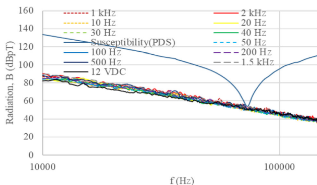
Fig. 7 Magnetic field emissions from side 3 of the motor shielded with one layer of aluminum foil of 0.0508-mm or 0.002-in. thickness
