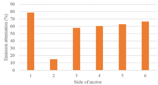
Fig. 10 Comparison of the average emission attenuations of six sides of the motor shielded with copper foil of 0.016256-mm (0.00064 in.) thickness at 73 kHz
