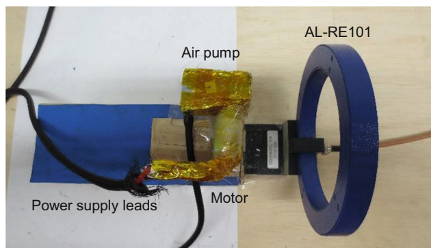
Fig. 6 Motor shielded with aluminum foil of 0.0508-mm (0.002 in.) thickness
