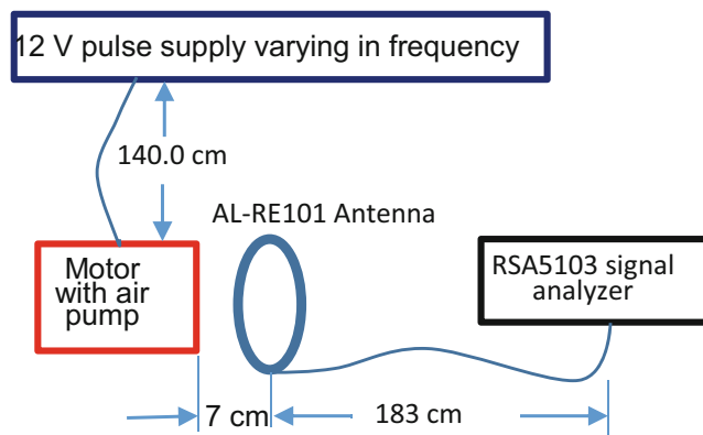
Fig. 1 Block diagram of the experimental setup for the PDM air pump motor
