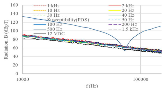
Fig. 5 Comparing magnetic field emission from side 3 of the motor having no shielding to the susceptibility of a PDS
