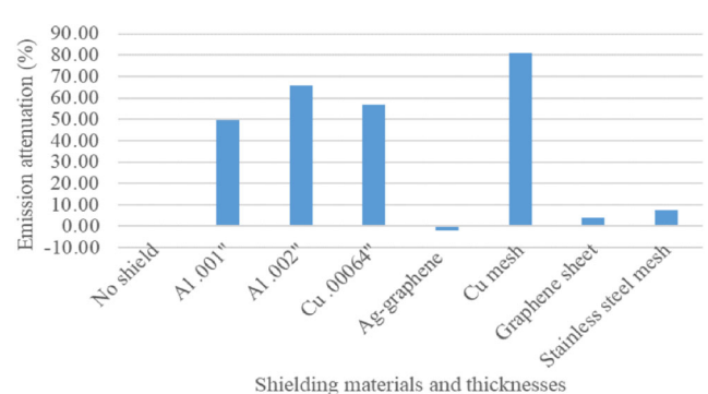
Fig. 11 Comparison of the average emission attenuations by the shielding materials and their thicknesses on all of six sides of the motor at 73 kHz
