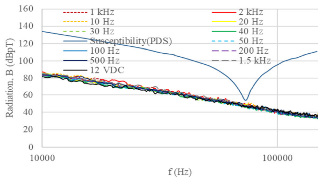
Fig. 8 Magnetic field emission from side 3 of the motor shielded with an enclosure of one layer of copper mesh with wire diameter of 0.1143 mm (0.0045 in.) and opening of 0.1397 mm (0.0055 in.)
