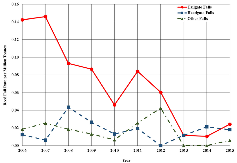
Fig. 3 Roof falls rates that resulted in a gateroad blockage or other nearby fall
