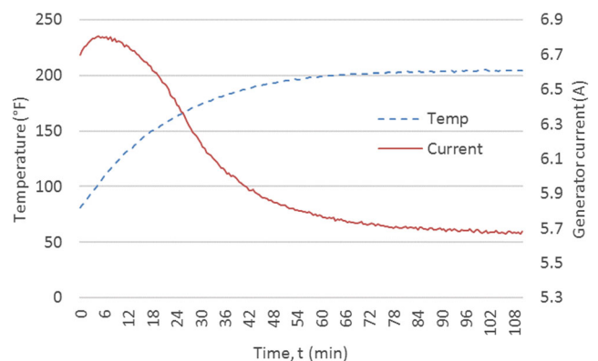
Fig. 3 Change of current with temperature for the generator running with continuous current in RMS value
