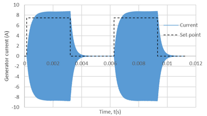
Fig. 6 Measured 73-kHz-current waves and set points for a set of dual pulses
