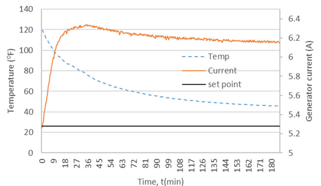
Fig. 7 The change of the generator current with temperature with the current initially set at 5.278 A in RMS value
