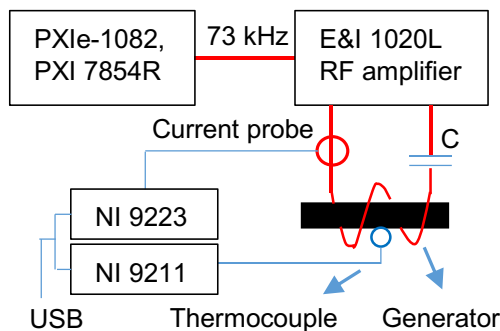
Fig. 1 Block diagram of the system instrumentation for the experiment
