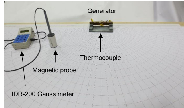
Fig. 2 Generator, gauss meter, and thermocouple used in the experiment
