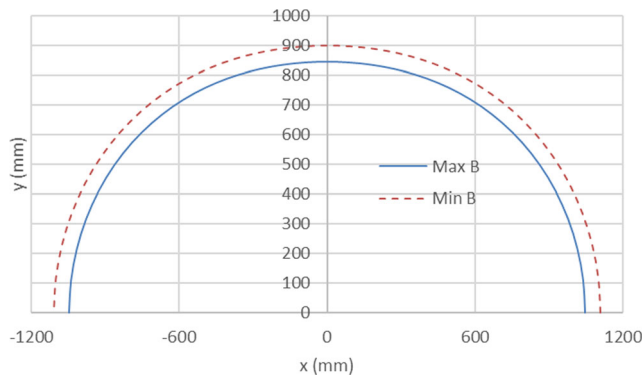
Fig. 4 Magnetic shells with maximum and minimum magnetic flux densities, B , associated with maximum and minimum generator current
