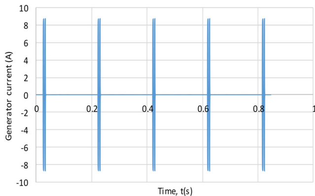
Fig. 5 A series of sets of two modulated pulses with a frequency of 73 kHz for the peak-to-peak current
