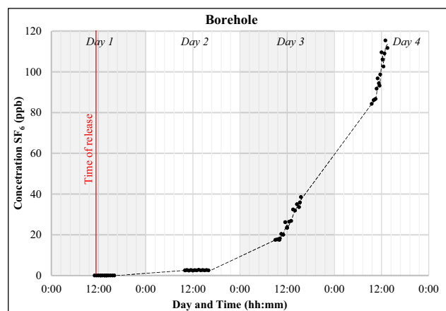
Fig. 9 Increasing concentrations of SF 6 measured at the surface borehole site during the gob test
