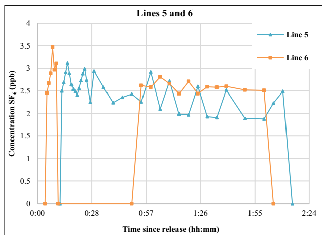
Fig. 5 Tracer gas concentrations determined for sampling during face test over test duration, sample lines 5 and 6. The arrival and peak occurred on line 6 located inby the face in the former, first tailgate gateroad, prior to the arrival and peak on sample line 5 at shield 177
