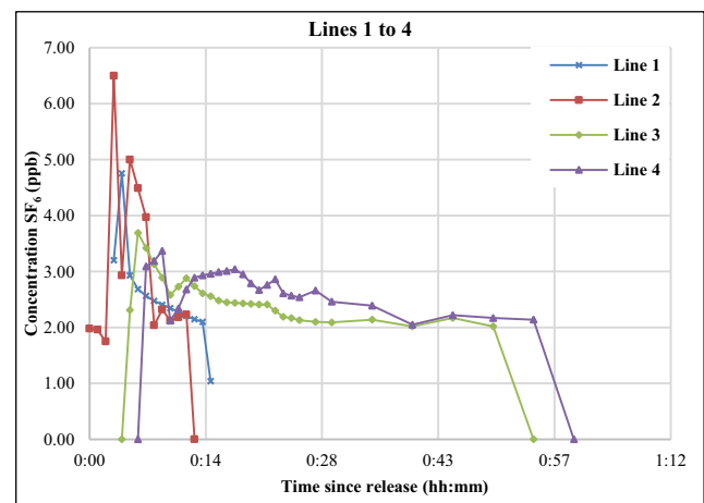
Fig. 4 Tracer gas concentrations determined for sampling during face test over test duration, sample lines 1 through 4. First arrival and peak occurred on line 2, prior to arrival and peak on sample line 1
