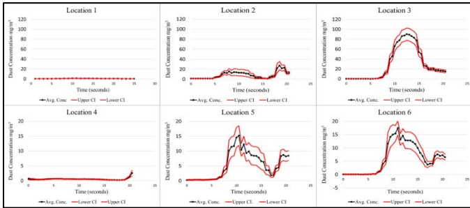
Figure 4. Coal dust—low air velocity baseline.
