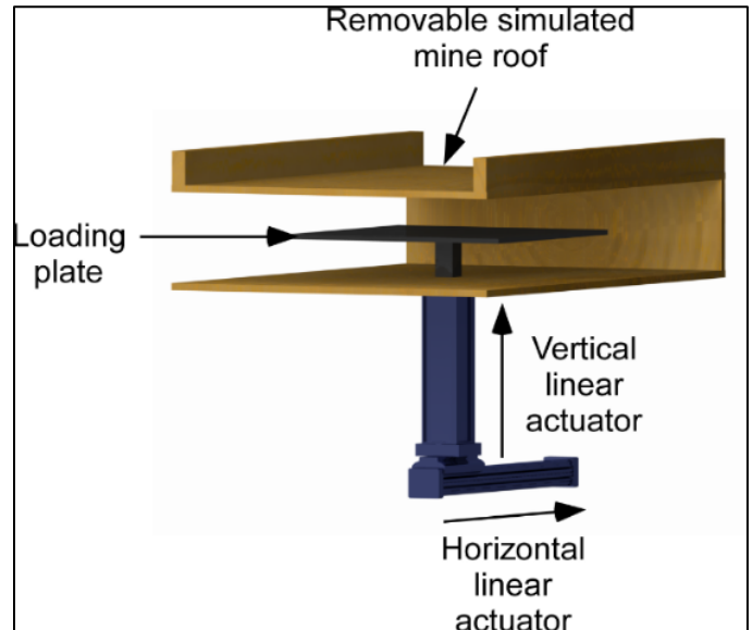
Figure 3. Test section 3D view.
