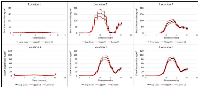
Figure 5. Coal dust—high air velocity baseline.
