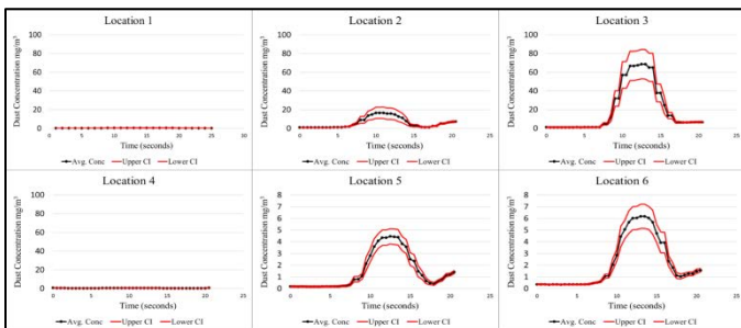
Figure 6. Limestone dust—low air velocity baseline.
