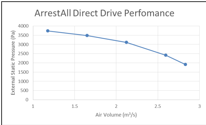
Figure 2. Baghouse fan performance curve.
