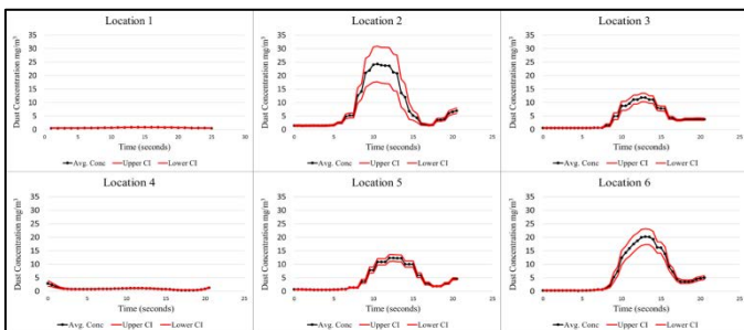
Figure 7. Limestone dust—high air velocity baseline.
