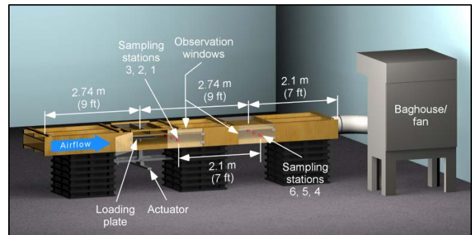
Figure 1. 3D schematic of the shield dust simulator. Sampling locations are located downwind of the loading plate and actuator, the location where the simulated shield movement takes place.
