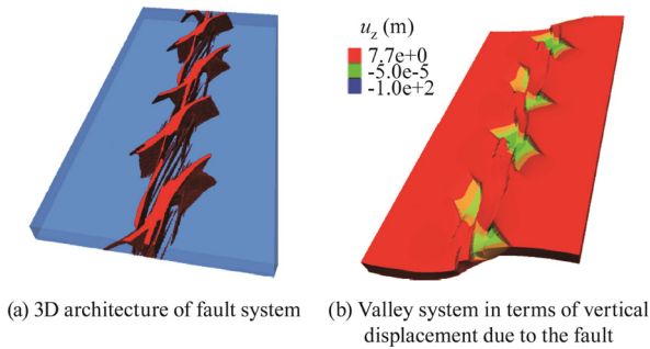
Fig. 3. Fault system and the induced displacement simulated by Chemenda et al. [11].
