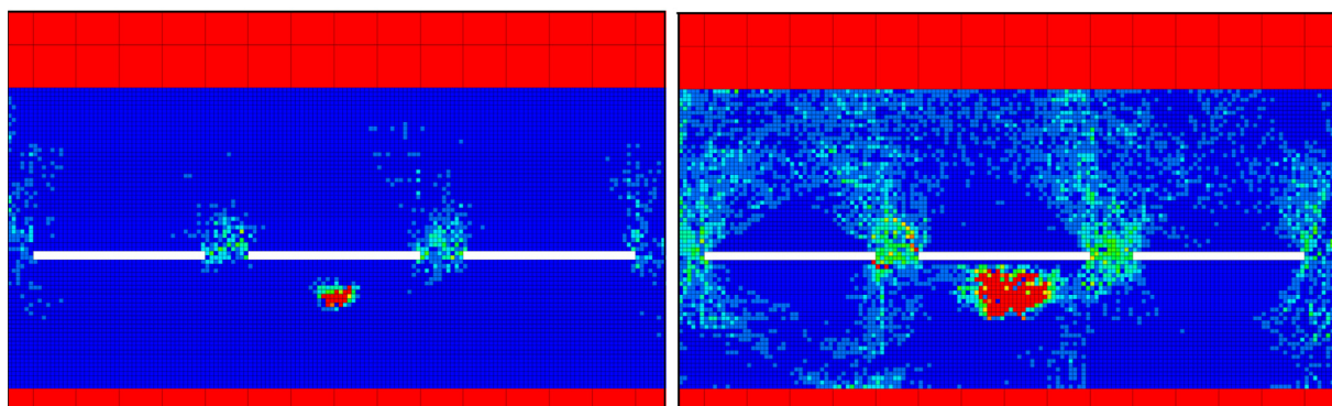
Fig. 7. Contours of plastic dissipated energy after excavation of each panel at the different stages of the fault.
