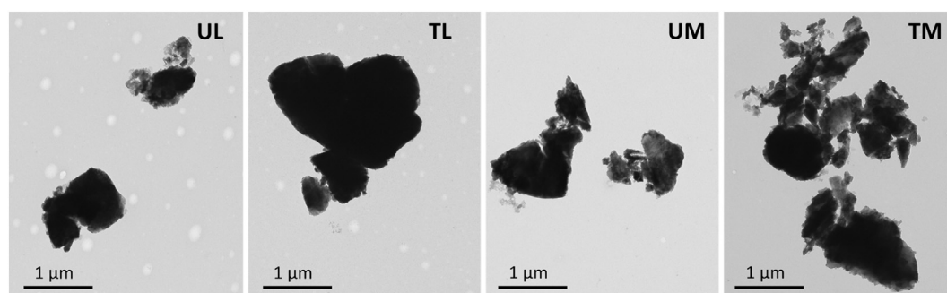
Fig. 2. Representative TEM images of respirable rock dust samples. UL - untreated limestone, TL – treated limestone, UM – untreated marble, TM – treated marble.
