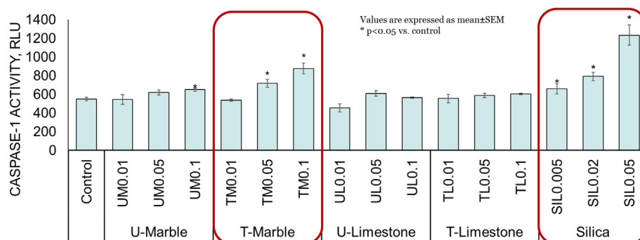
Fig. 5. Intracellular caspase-1 activity following 24 h exposure to various concentrations of rock dusts and crystalline silica in THP-1 cells. Values are expressed as mean \pm SEM. *p < .05 vs. control.
