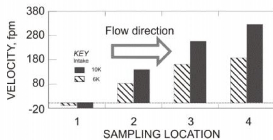
Figure 11. Air speed across face in 16-1/2 ft entry, 2 ft from face
