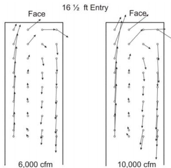
Figure 7. Flow profiles in 16-1/2 ft entry
