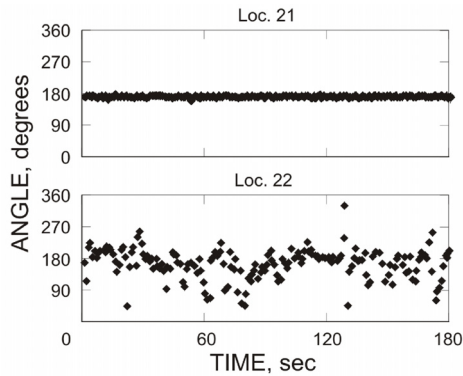
Figure 12. Flow direction at two locations
