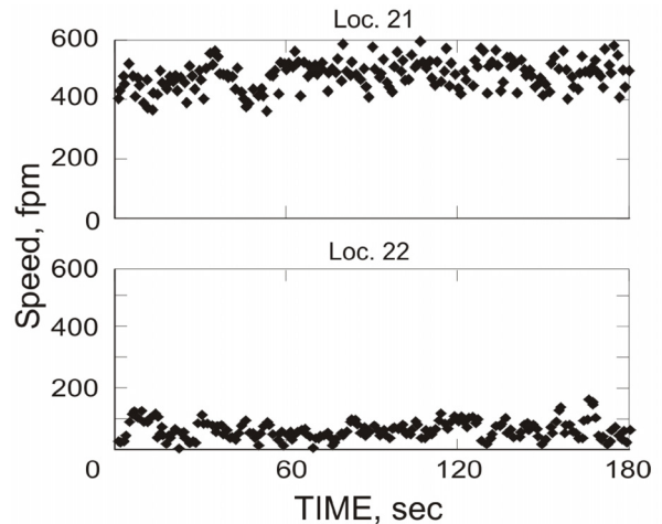
Figure 13. Speed measurements at two locations
