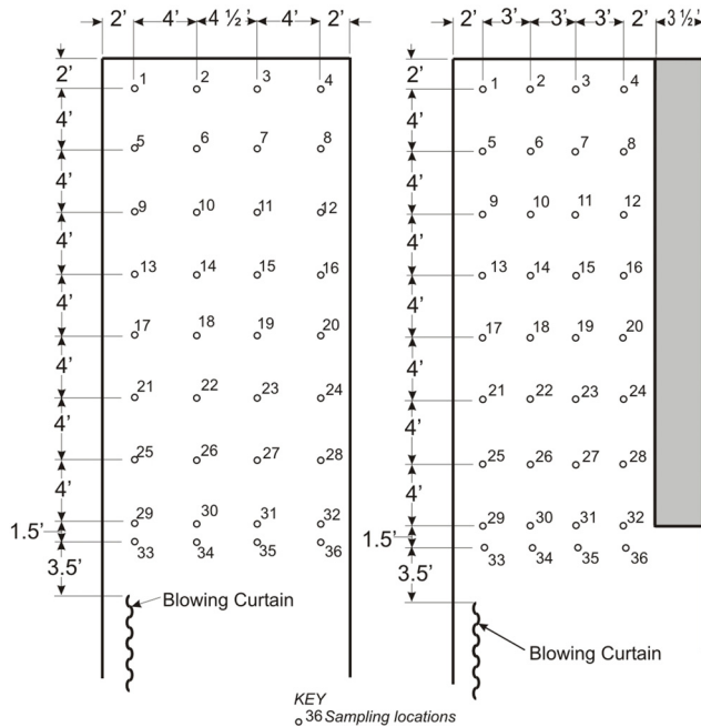
Figure 5. Measurement locations in gallery
