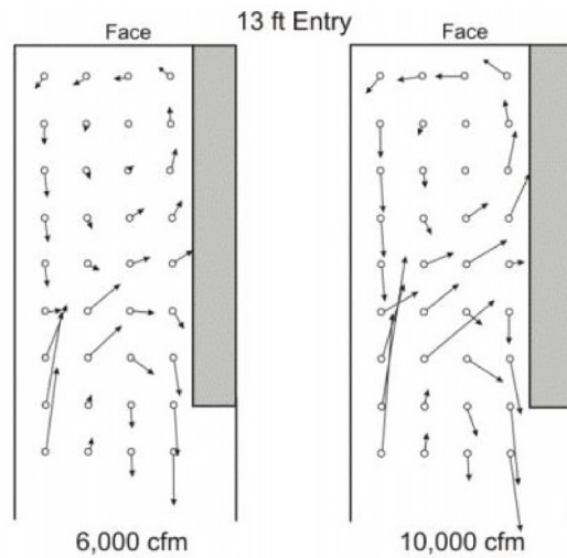
Figure 6 Flow profiles in 13ft entry
