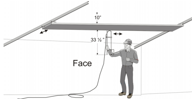
Figure 3. Support system for moving anemometer
