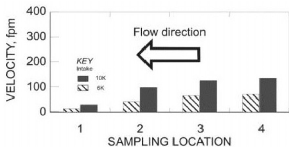
Figure 10. Air speed across face in 13 ft entry, 2 ft from face
