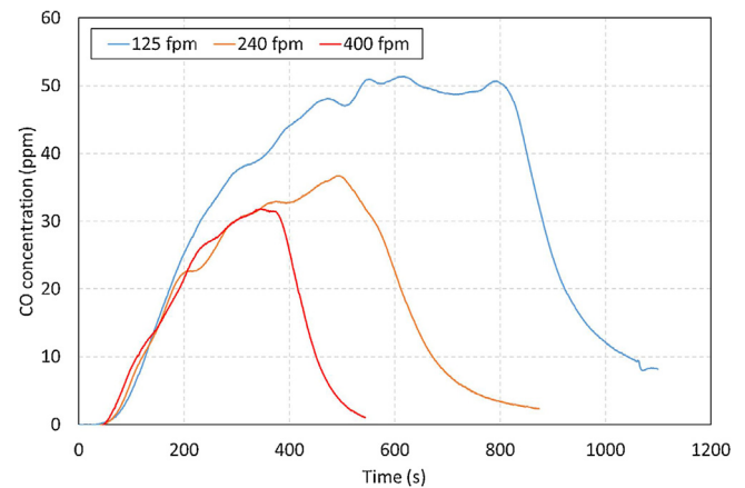
Fig. 4. CO concentrations with different airflow velocities.
