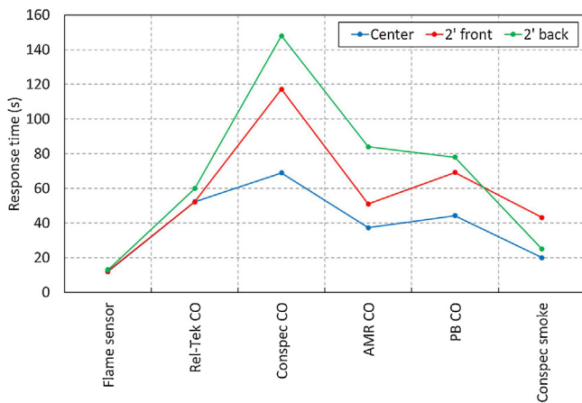
Fig. 10. Sensor response time comparison between CO, smoke, and flame sensors: small diesel fire.
