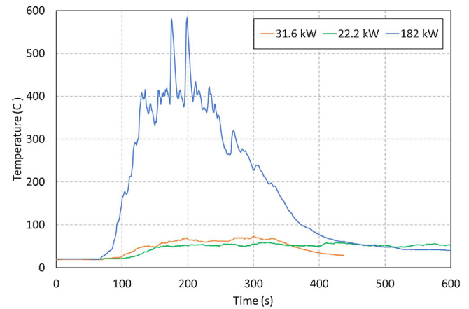
Fig. 12. Gas temperatures with different heat release rates.
