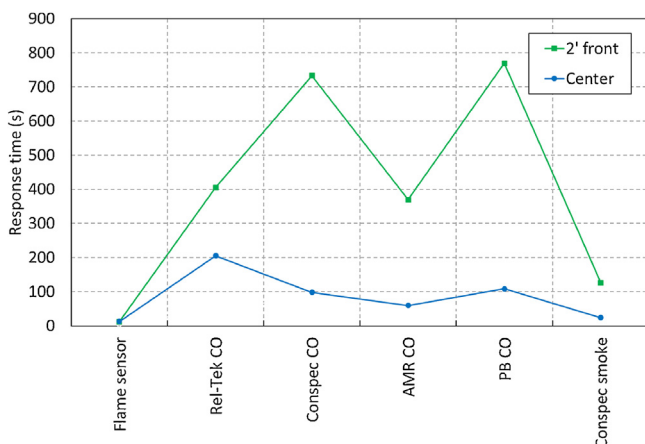
Fig. 11. Sensor response time comparison between CO, smoke, and flame sensors: large diesel fire.
