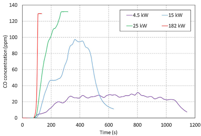
Fig. 6. CO concentrations with different heat release rates.
