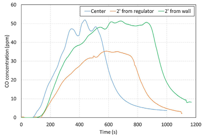
Fig. 5. CO concentrations with different fire locations.
