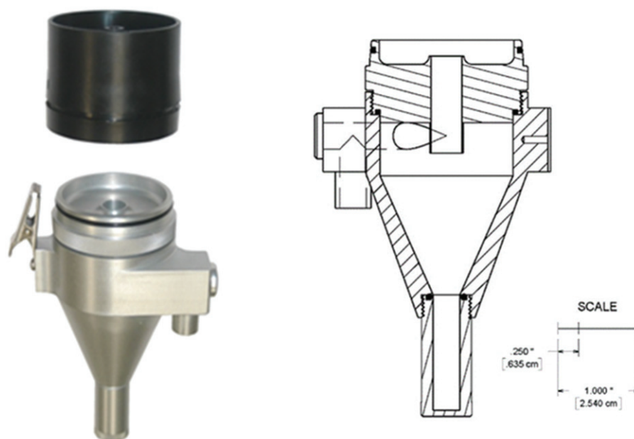
Figure 1. GK4.162 cyclone and its cutway drawing (courtesy of BGI Inc.).
