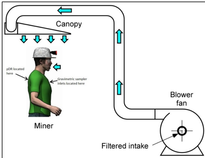
Figure 4. Locations of gravimetric sampler inlets and pDR sampler with respect to the roof bolter operator.
