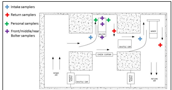
Figure 3. Locations of sampling packages for testing the dust control efficiency of the roof bolter canopy air curtain.
