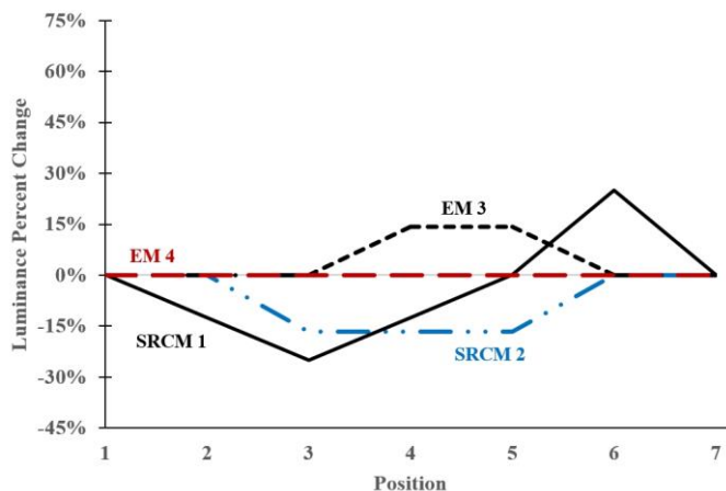
Fig. 5. The luminance percentage change, with respect to position 1, for the various photometer position at each rib location. The measurement distance was 0.6 m (2 ft).
