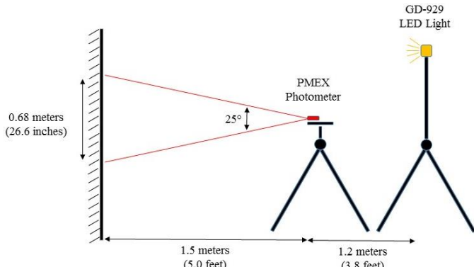
Fig. 1. General layout of the photometer and light source with respect to the mine rib. The light source was placed directly behind the photometer and positioned normal to the coal rib.
