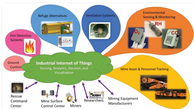
Figure 2 Example of IIoT system in coal mines.
