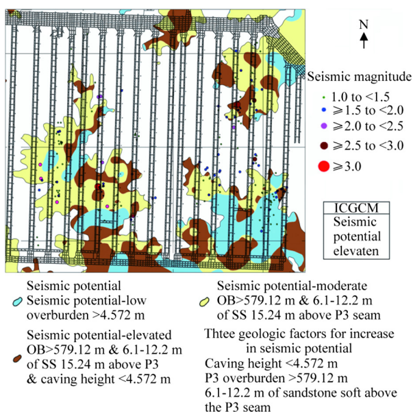
Fig. 6. Seismic potential map.
