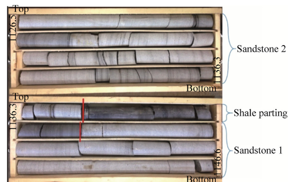
Fig. 2. Core from Sandstone 1, shale parting, and sandstone.
