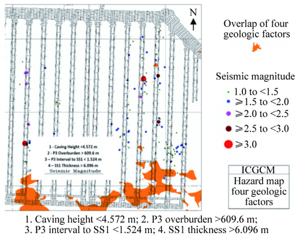
Fig. 5. Mining hazard map.
