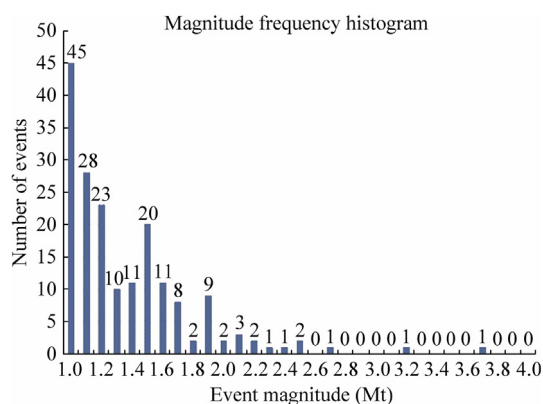
Fig. 3. Magnitude frequency histogram.
