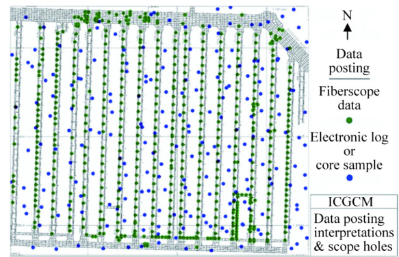
Fig. 4. Geological data points.
