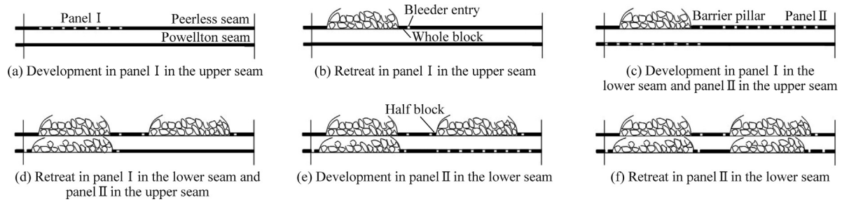
Fig. 4. Sequence of development and retreating in the upper and lower seams.
