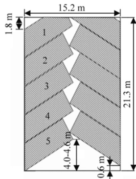
Fig. 18. Pillaring plan in the lower seam.
