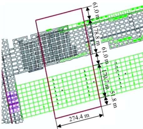
Fig. 6. Modeled area in the lower seam.
