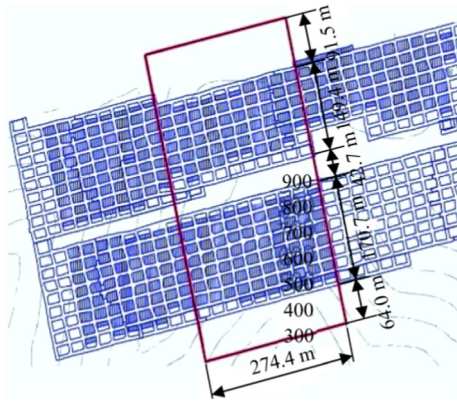
Fig. 5. Modeled area in the upper seam.
