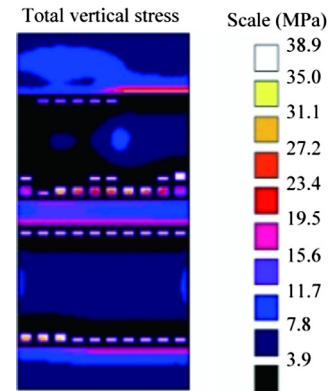
Fig. 7. Vertical stress distribution over the retreat panels in the upper seam.
