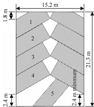
Fig. 14. Pillaring plan in the upper seam.
