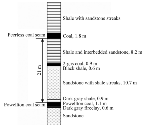
Fig. 2. Geological column of the interburden strata.
