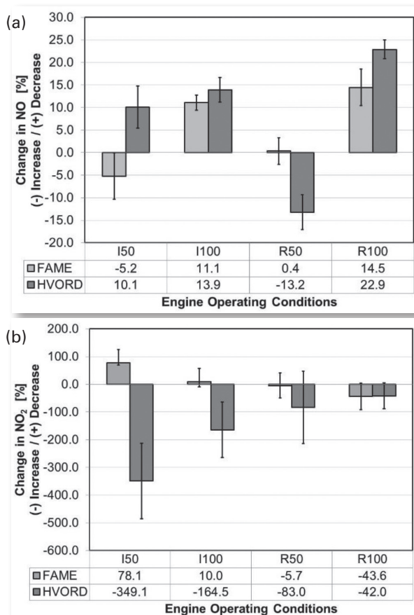
Effects of the tested fuels on (a) NO and (b) NO 2 concentrations.
