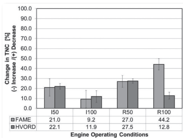
Effects of the tested fuels on the total number concentrations (TNC) of aerosols.
