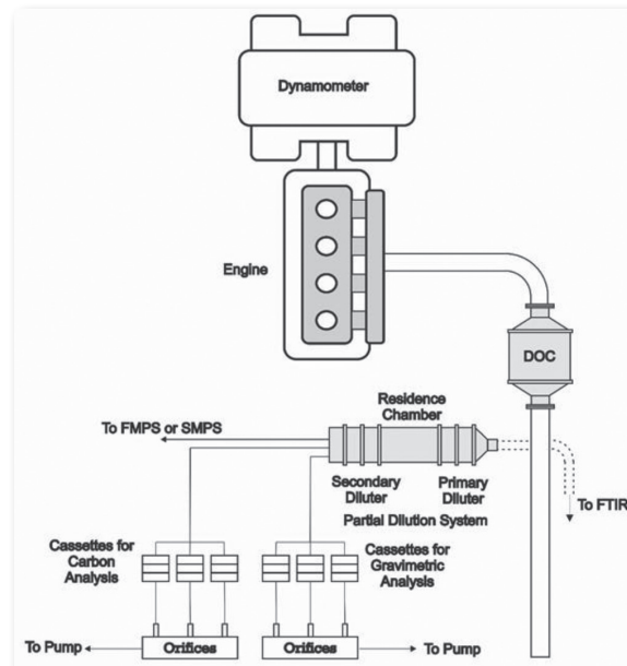
Figure 1 Experimental layout.
