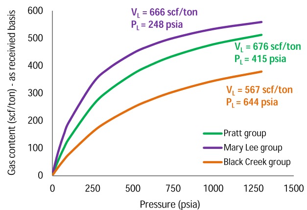
Fig. 9. Langmuir isotherms and their parameters determined for each of the coal groups.
