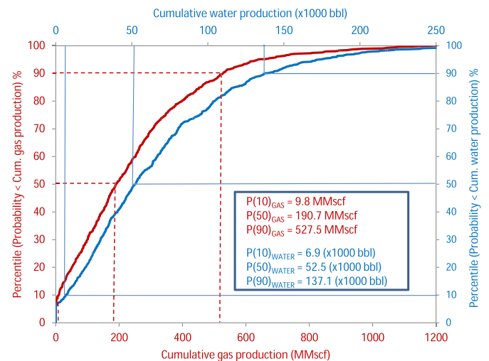
Fig. 20. Cumulative frequency histogram of gas and water productions estimated using the values in Table 4 with a stochastic approach. The percentile values are given in the inset table.
