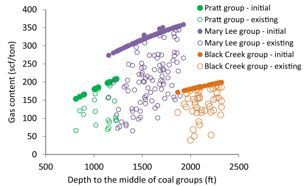
Fig. 14. Calculated initial gas contents of the coals using initial pressures and the isotherms given in Fig. 9. Circles are existing gas contents based on existing pressures.
