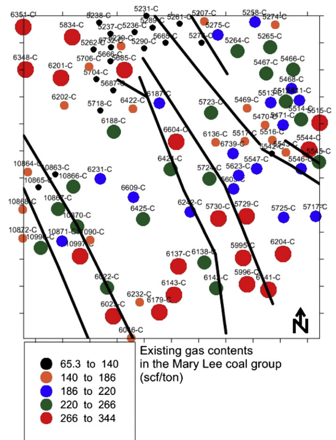
Fig. 15. Spatial distribution of predicted existing gas contents within the Mary Lee coal group in the study area. In the sorted class map, symbol sizes were scaled according to their magnitude.
