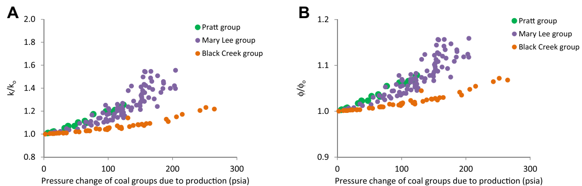
Fig. 17. Fractional changes in permeability (A) and porosity (B) in coal groups compared to initial values as a result of matrix shrinkage. Presented data points correspond to each of the well locations in the study area.
