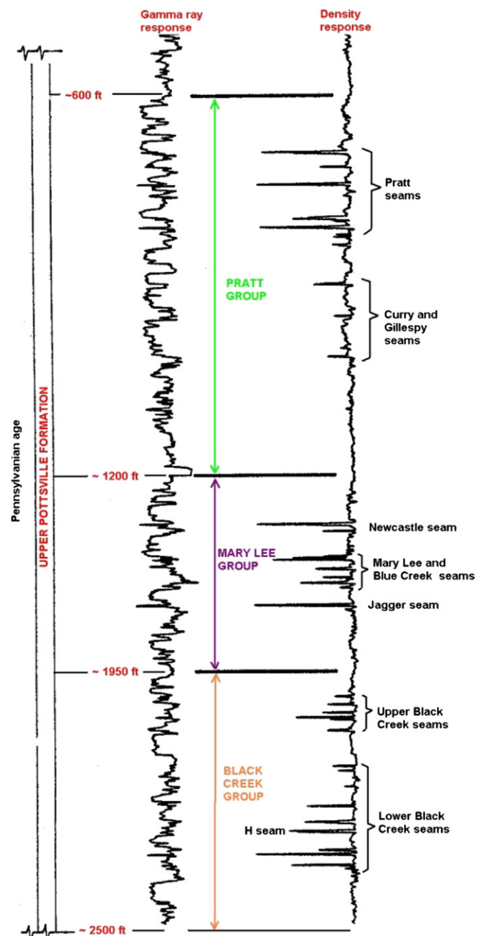
Fig. 2. A typical well log showing gamma ray and density log responses of Upper Pottsville coals. The figure also shows the seams within each coal group and their approximate depth intervals within the study area.
