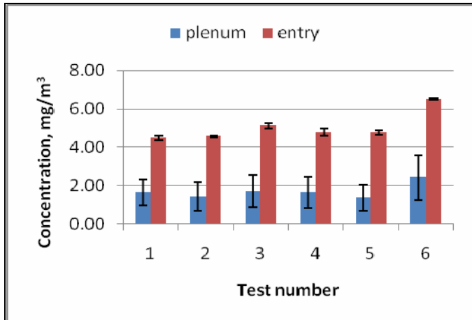
Figure 13. Relative dust concentrations, showing standard error bars—under the plenum versus outside the plenum (i.e., entry).
