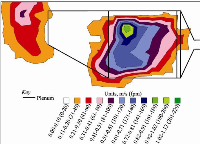
Figure 6. Velocity profile of original CAC design.
