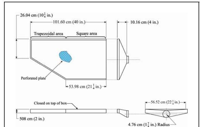
Figure 4. Original air curtain designed for a roof bolter canopy.
