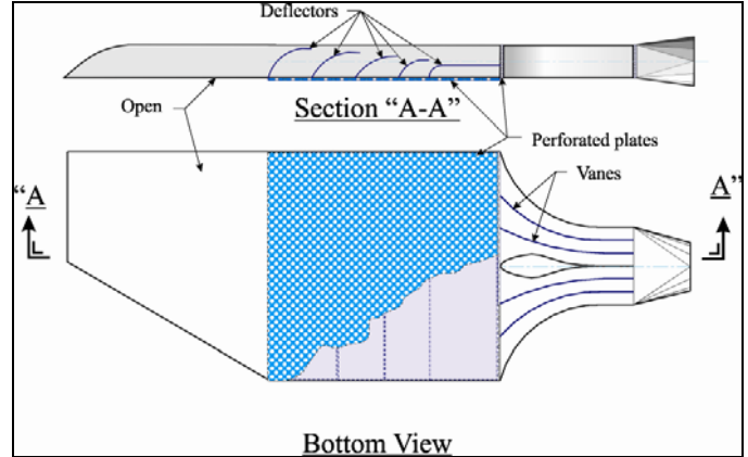
Figure 7. Prototype modified based upon CFD analysis.
