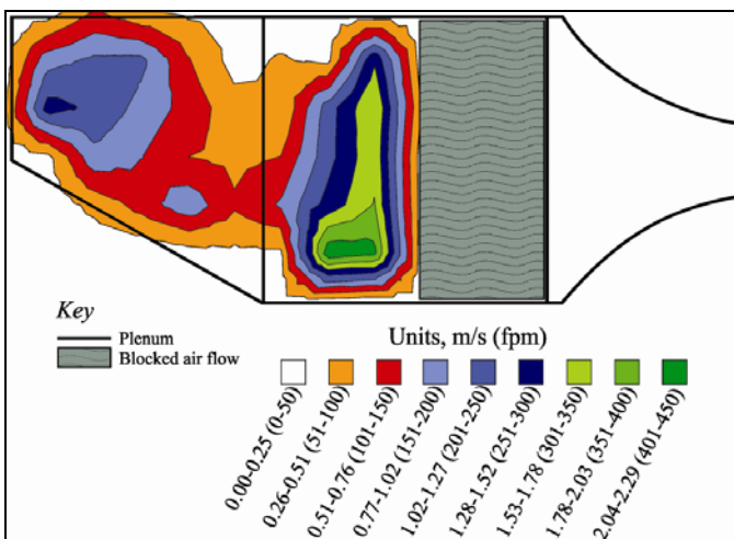
Figure 9. Velocity profile of the final design.
