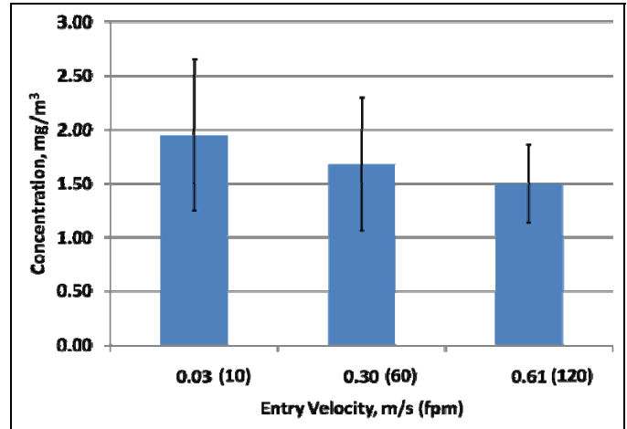
Figure 14. Dust concentration averages for three test velocities showing standard error bars.
