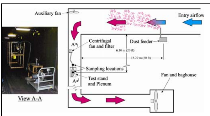
Figure 10. NIOSH mine gallery test setup configuration.
