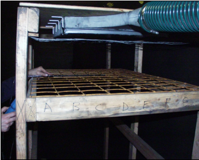
Figure 5. Velocity measurement grid 25.4 cm (10 in.) beneath the plenum.
