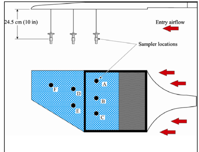
Figure 11. Dust sampling instrument locations under plenum.
