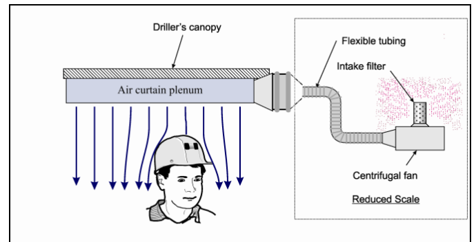
Figure 2. Roof bolter operator protected by clean airflow provided by canopy air curtain.
