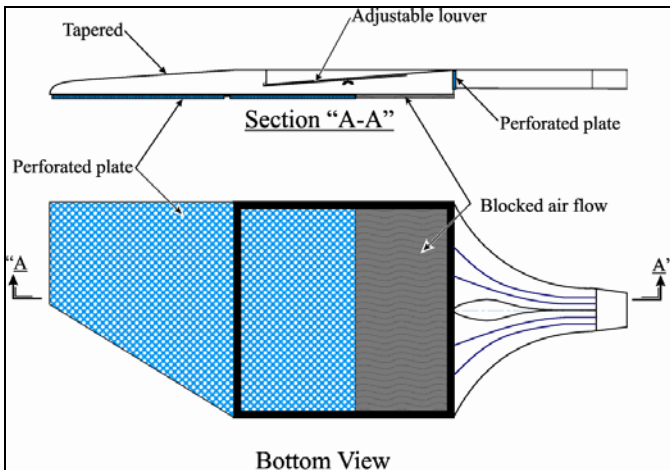
Figure 8. The final CAC design.
