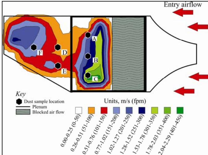
Figure 12. Dust samplers relative to air velocity under plenum.
