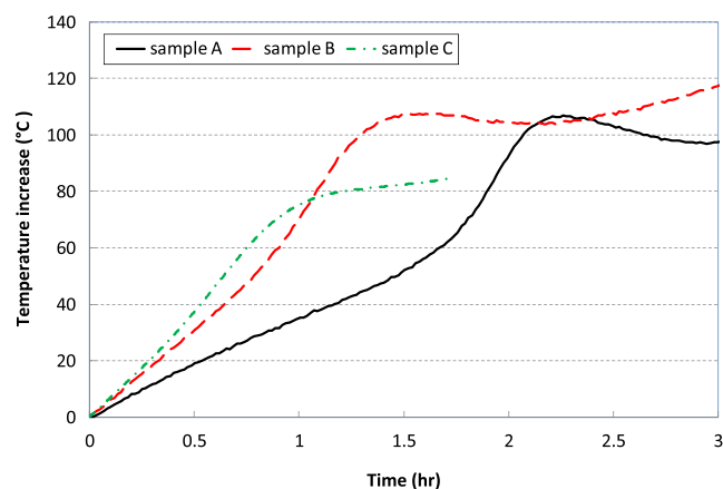
Fig. 9. Center coal temperature rises for three samples under the airflow rate of 300 cm³/min.
