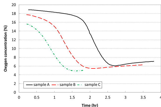
Fig. 10. Oxygen concentrations for three samples under the airflow rate of 300 cm³/min.
