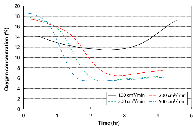
Fig. 6. Oxygen concentration at the exit of the oven under different ventilation rates for sample B.
