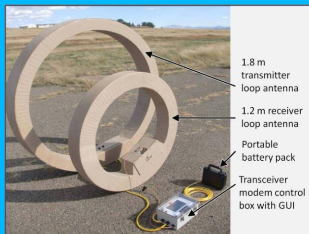
Fig. 5. Integrated Stolar surface transceiver with antennas
