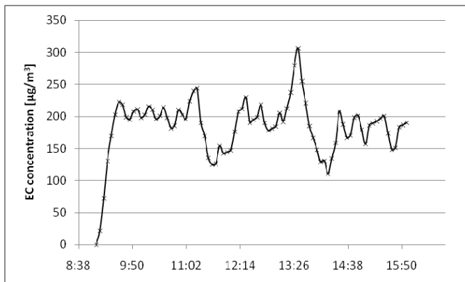
Figure 6 A real-time trace of recorded EC taken downstream during an isolated zone test. The chart shows concentration oscillations ascribed to the movement of the vehicle throughout the test.
