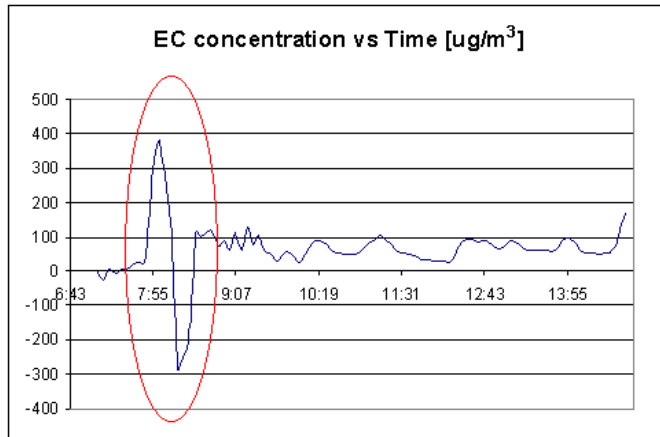
Figure 2 A chart of EC concentration vs. time, showing temperature interference at 07:50-08:15.
