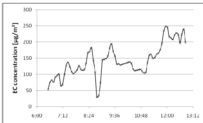
Figure 5 A chart showing a fluctuating, but overall increase in recorded EC concentration from 75 to 200 \mu\text{g}/\text{m}^3 throughout a six hour time frame.
