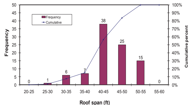
Figure 1. Distribution of roof span dimensions measured at 34 different underground stone mines.
