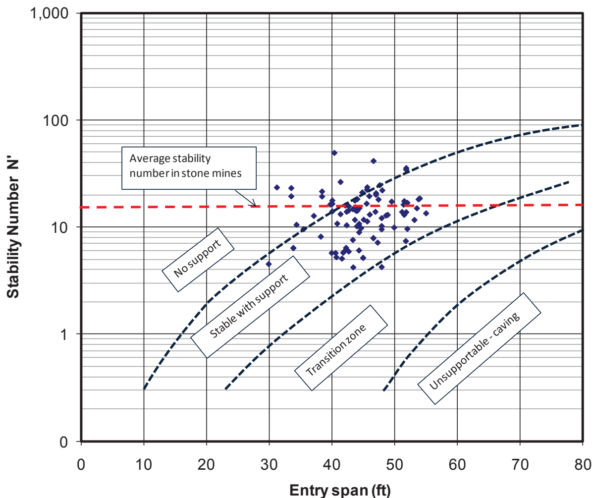
Figure 5. Stability chart showing stone mine case histories and stability zones, modified after Matthews et al. (1980), Potvin (1988), Nickson (1992), and Hutchinson and Diederichs (1996).
