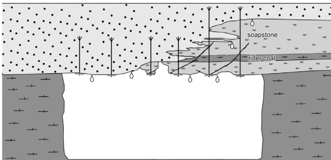
Figure 35: Hazardous roof conditions occur on the margins of a sandstone channel at a West Virginia mine.
