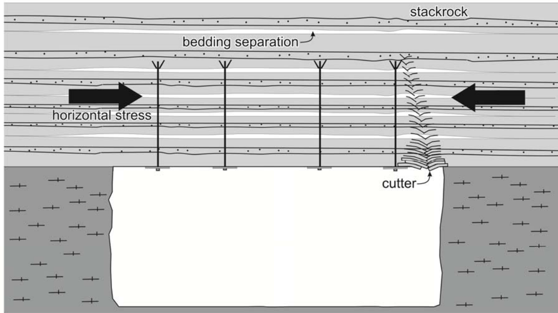
Figure 2: Stackrock delaminates and cutters form when roof is subjected to horizontal stress
