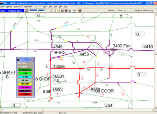
Figure 3 Visualization of fire area (carbon monoxide levels) during the early stages of contamination.
