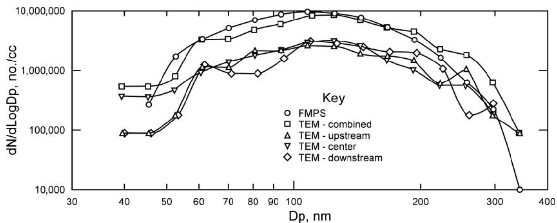
FIG. 13. Comparing particle size distribution of the original aerosol (FMPS measured) with results of TEM analysis of particles at upstream, center and downstream locations on the sample.
