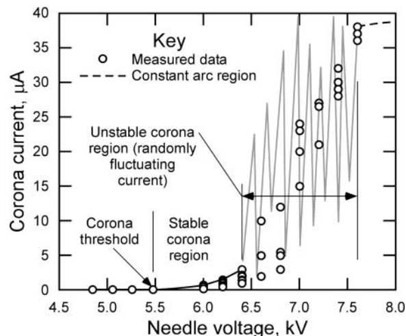
FIG. 3. Measured ion current versus corona voltage during prototype ESP testing.
