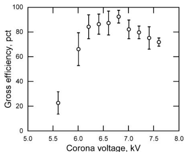
FIG. 11. Gross collection efficiency (measured by CPC) versus corona voltage using the ESP of Figure 5 operating at 55 cc/min flow rate.
