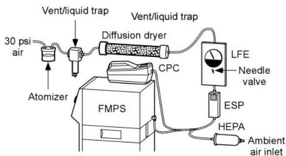
FIG. 6. Schematic of experimental setup for evaluating collection efficiency of the ESP.
