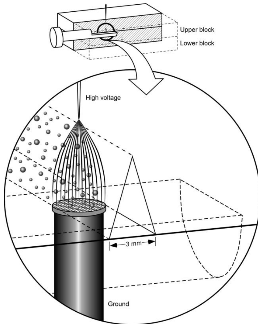
FIG. 2. Schematic of the collection region of the prototype ESP.
