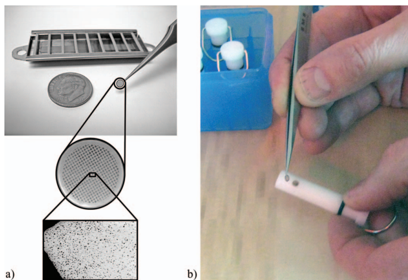
FIG. 4. (a) Tweezers are used to handle grids and a radiation source (background) helps to prevent static charge. (b) Sample media is placed onto the ground post of a key for use in the ESP (sealable case for keys in background).
