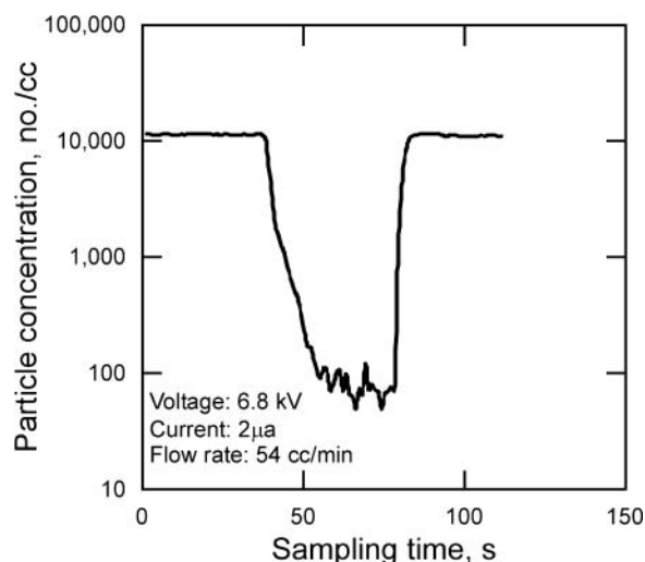
FIG. 7. Particle concentration versus time for a typical test, measured with the CPC.
