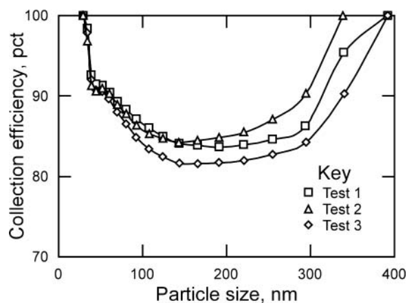
FIG. 8. Size-dependent gross collection efficiency of NaCl particles, measured with the FMPS, for a prototype ESP similar to that in Figure 5, operating at 100 cc/min flow rate and 6.4 kV corona voltage.
