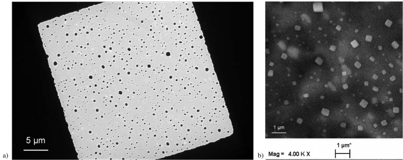
FIG. 12. Examples of NaCl particle deposition onto: (a) TEM grid (b) aluminum foil media (SEM image).
