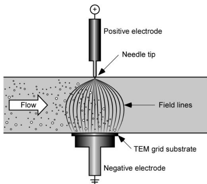
FIG. 1. Point to plane ESP configuration.
