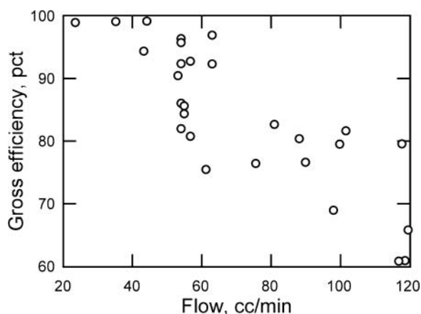
FIG. 10. Gross efficiency (measured with CPC) versus flow rate for prototype ESP operating at 6.4 kV.
