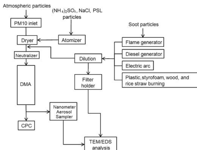
FIG. 1. A schematic outline of the experimental setup (DMA: Differential Mobility Analyzer, CPC: Condensation Particle Counter, TEM: Transmission Electron Microscopy, EDS: Energy Dispersive Spectroscopy).
