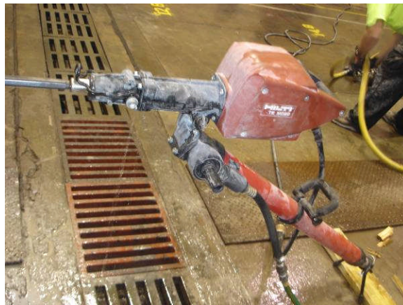
(c) Hilti TE MD20.
