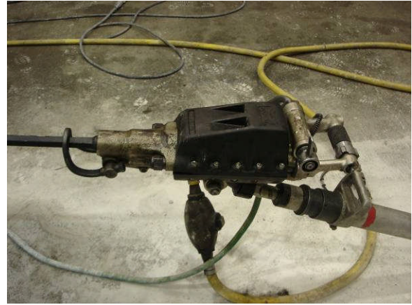
(b) Gardner Denver S83 with muffler.
