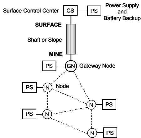
Fig. 8. Arrangement for a wireless-mesh system.
