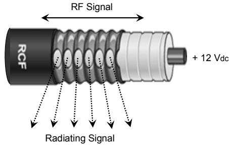
Fig. 1. Leak-feeder cable.
