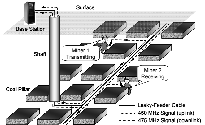
Fig. 2. Basic operation of the enhanced leaky-feeder system.
