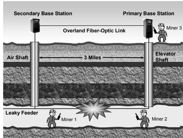
Fig. 5. Redundant path established by a surface, overland link.
