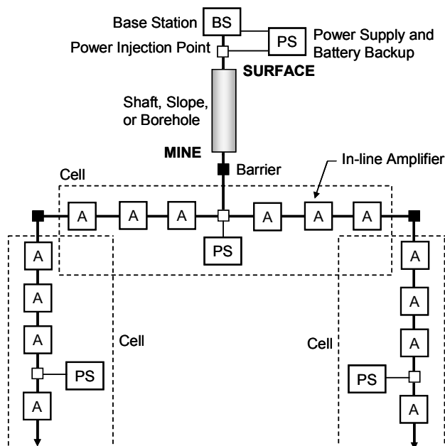
Fig. 3. General arrangement of a leaky-feeder system.
