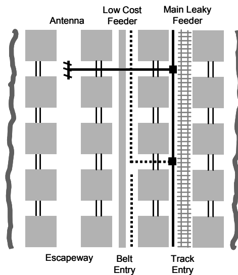
Fig. 4. Extended communications coverage.
