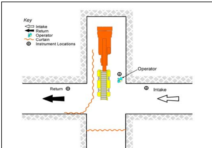
Figure 2. Sampling package locations for a typical cut on an exhausting ventilation scheme.
