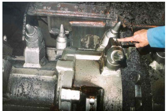
Figure 1b. Wet head sprays on continuous miner cutter head.
