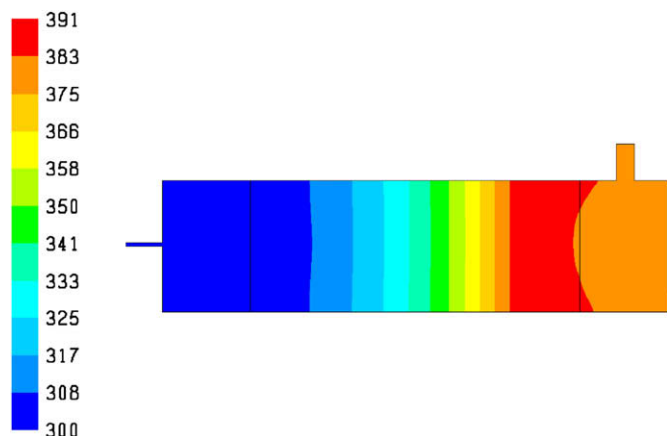
Fig. 5. Temperature distribution (K) in coalbed chamber and plenum areas at 24.6 days.
