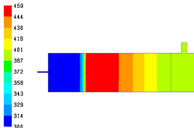
Fig. 7. Temperature distribution (K) in coalbed chamber and plenum areas at 25.6 days.
