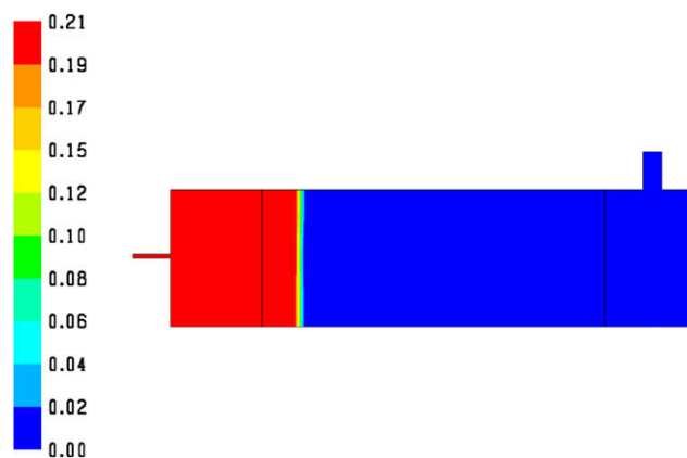
Fig. 8. Oxygen concentration distribution (1 = 100%) in coalbed chamber and plenum areas at 25.6 days.
