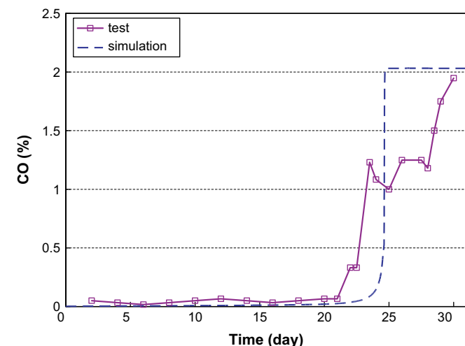
Fig. 14. Comparison between simulation and test for carbon monoxide concentration at exit.
