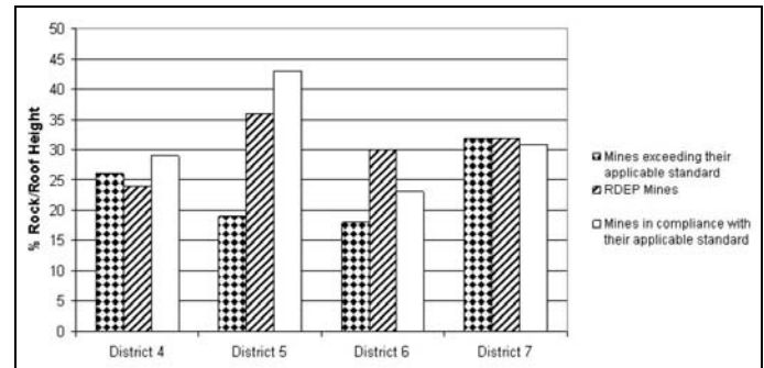
Figure 2. Percentage of rock cut to mine roof height for targeted mines.
