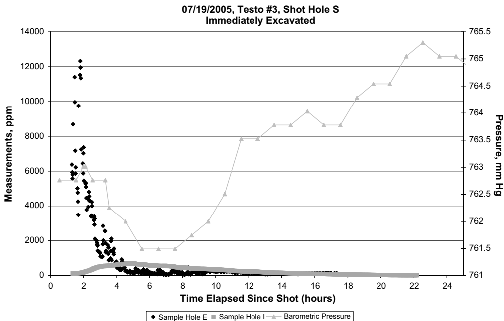
Fig. 8. CO measurements over time with immediate excavation.
