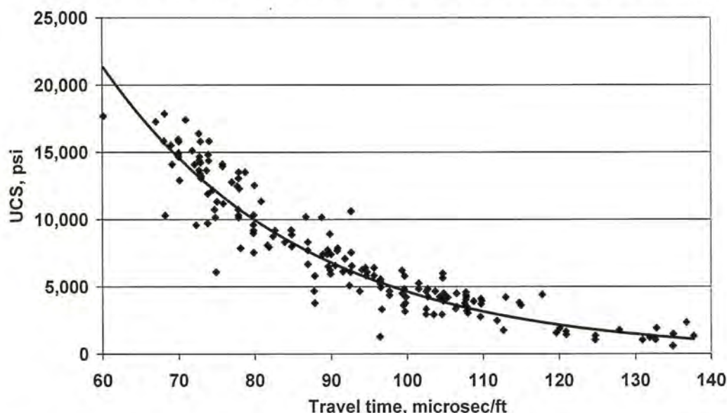
Figure 1. Sonic travel time versus UCS data from the Australian German Creek seam. Data after McNally (1987).
