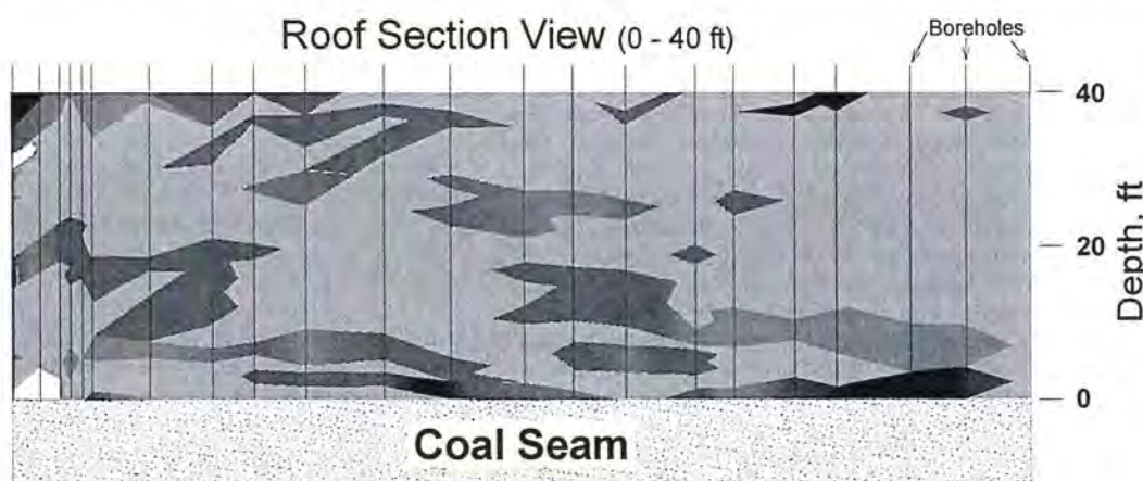
Figure 2. Contour plot of UCS of the immediate roof above a gateroad at the Crinum mine, Queensland, Australia (Payne, 2008). UCS data computed from sonic travel time log data, with black representing the weakest roof and light gray to white the strongest roof. Vertical scale 0 to 40 ft. Plot width approximately 8,000 ft (after Payne, 2008).
