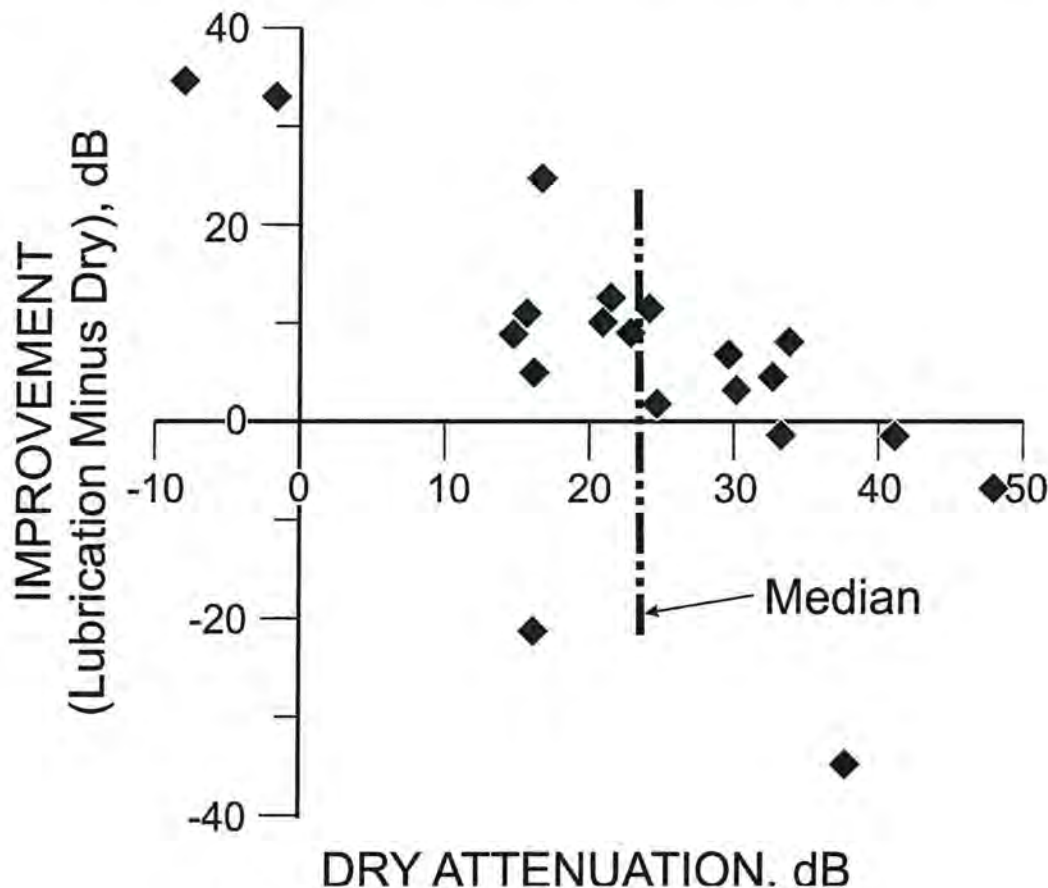
Figure 1: Improvement in attenuation from earplug lubrication
