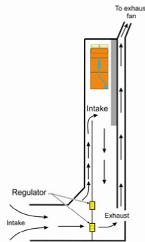
Figure 3. Ventilation test gallery.
