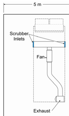
Figure 4. Model mining machine with scrubber.
