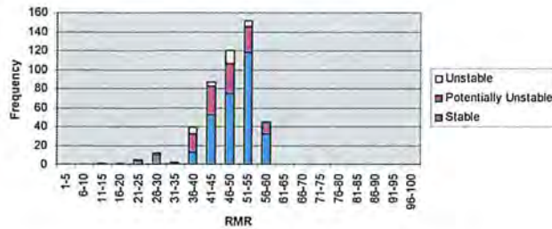
Figure 3: Weak Rock Database RMR 76 Distribution
