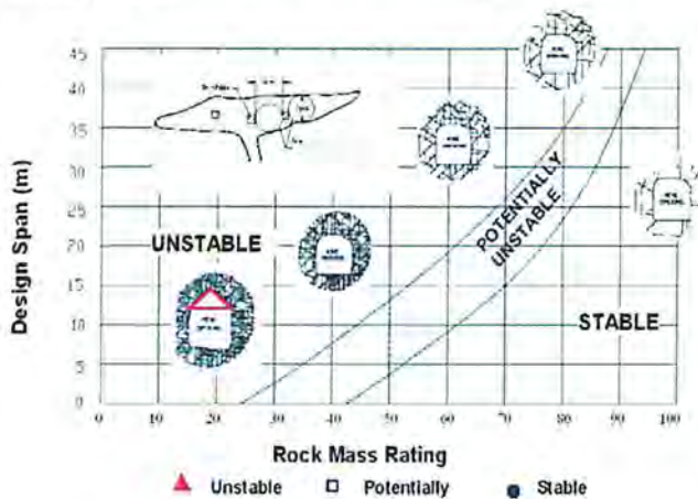
Figure 2: Updated Critical Span Curve
