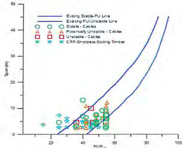
Figure 7: Category D points on Span Design Curve
