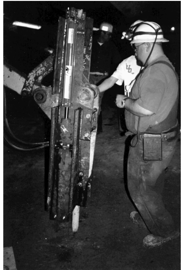
Figure 11.— Track-guided pincher arm attached to hydraulic impact hammer head.
