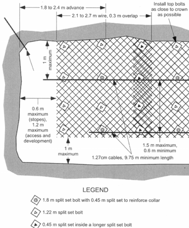
Figure 4.—Typical support scheme employed in rockbursting ground.
