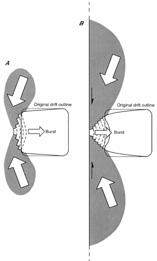
Figure 2.—Buckling of rock plates is driven by release of gravitational and elastic potential energy (A). A weak discontinuity can dramatically increase the amount of energy released, resulting in a more hazardous rockburst (B).
