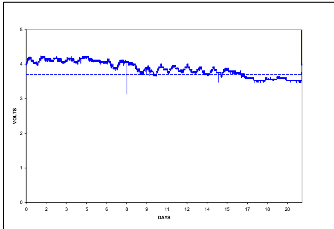
Figure 2. Beam sensor response in the main haulage way.
