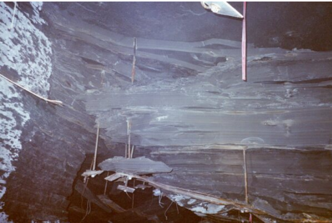
Figure 6. Roof fall in moisture-sensitive roof.
