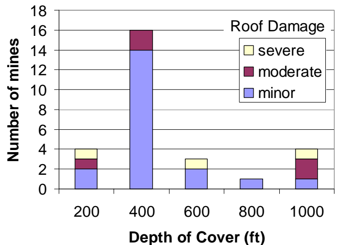
Figure 10. Distribution of Illinois Basin mines by depth of cover (bars include mines at all depths between that bar and the previous bar).
