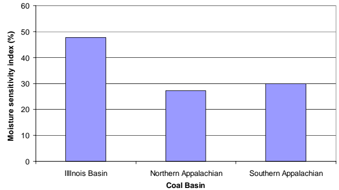
Figure 3. Average moisture sensitivity index of roof rocks in NIOSH database by basin.
