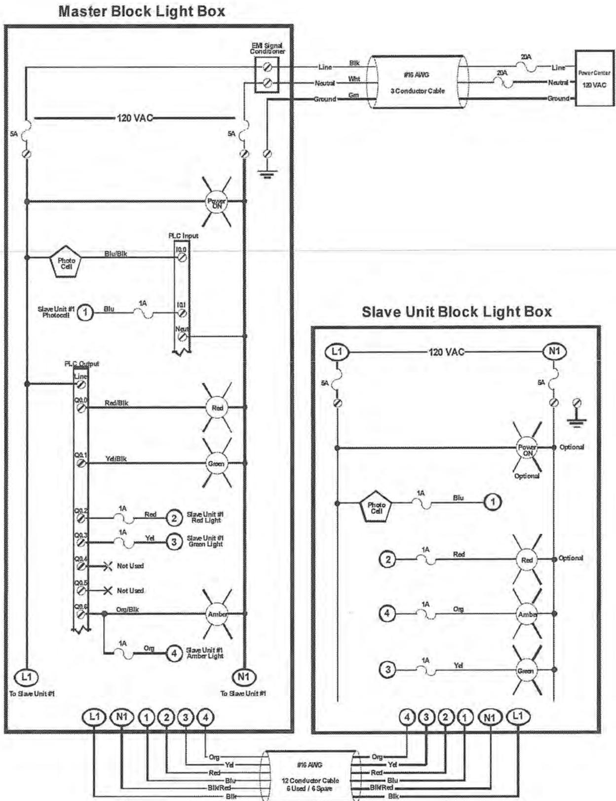
Fig. 1. Block light electrical circuit diagram.
