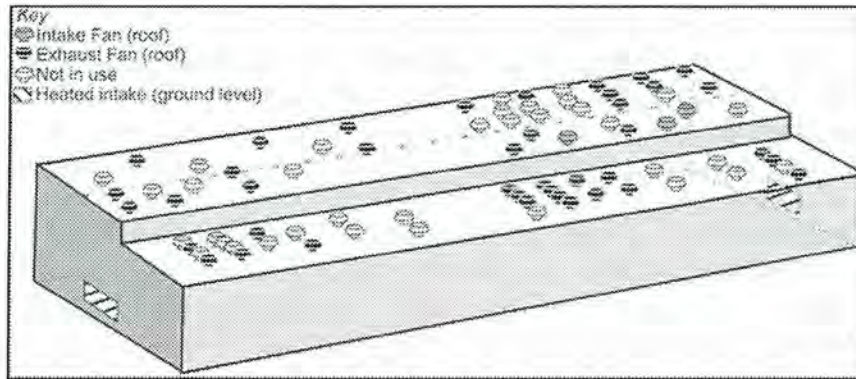
Figure 5. Roof fans at iron ore plant.
