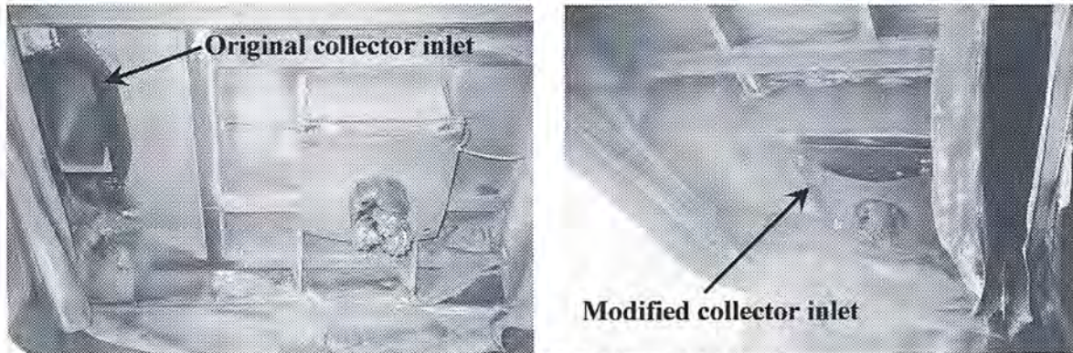
Figure 2. Original and modified collector inlet locations.
